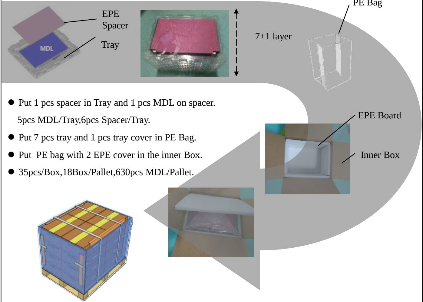
Figure 22. Packing Order
