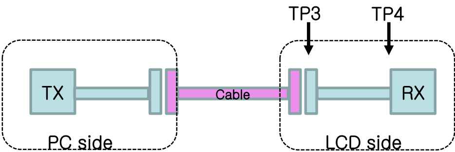
Mainlink eye diagram test point
