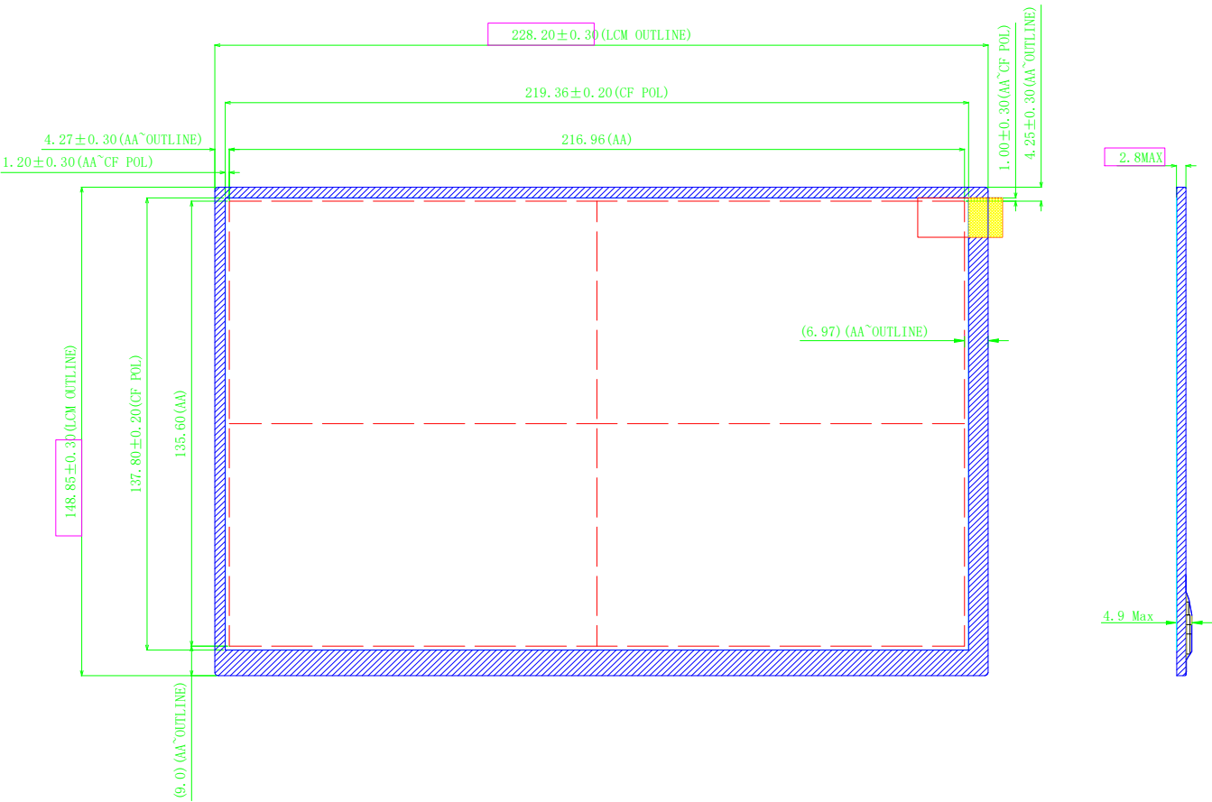
Figure 1. TFT-LCD Module Outline Dimension (Front View)
